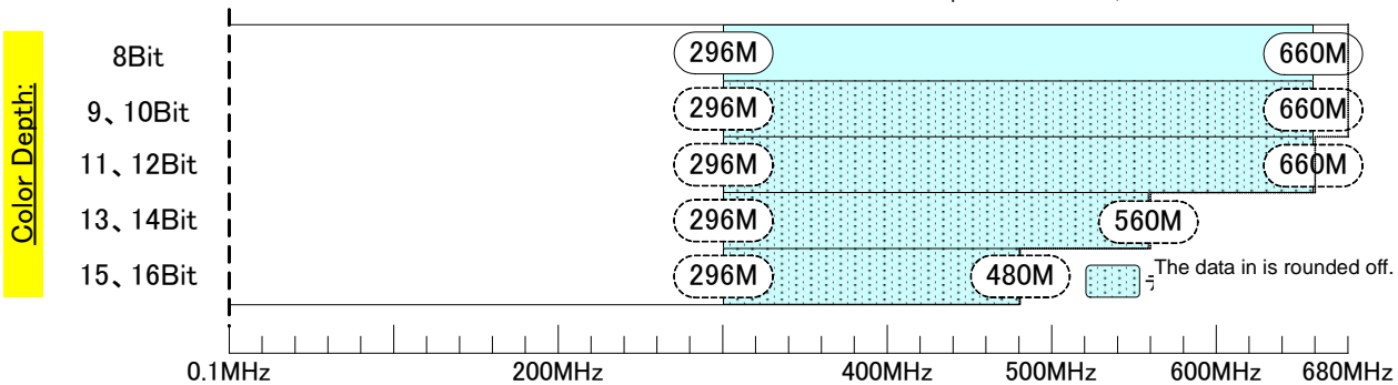
Restrictions on dot clock frequency for 4K2K( iTMDs) (DVI MODE/Quad Link)
