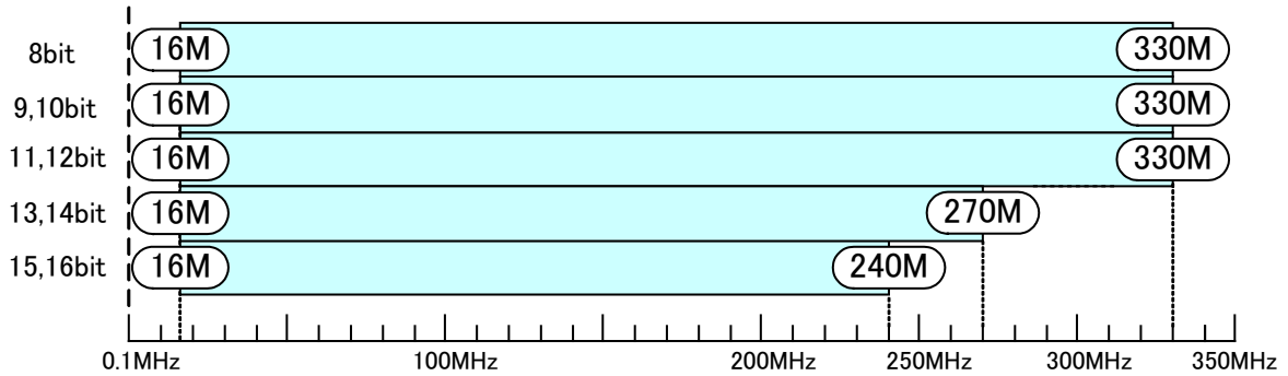
Restrictions on Dot Clock Frequency for DP1, DP2(Single Mode)
