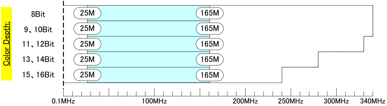
Restrictions on dot clock frequency for 4K2K(iTMDs) (DVI MODE/Single Link)
