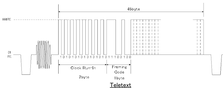
Teletext waveforms
