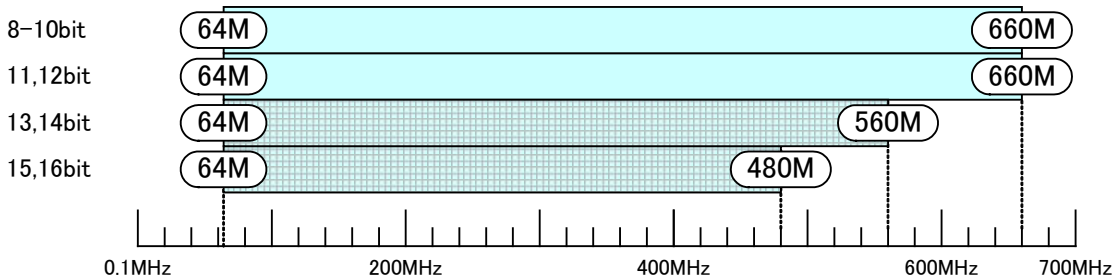
Restrictions on Dot Clock Frequency for DP1, DP2(Split Mode)
