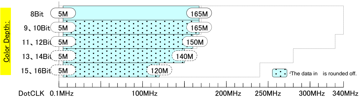
Restrictions on dot clock frequency for VGA
