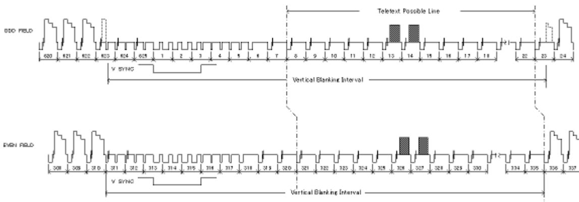
VBI waveforms
