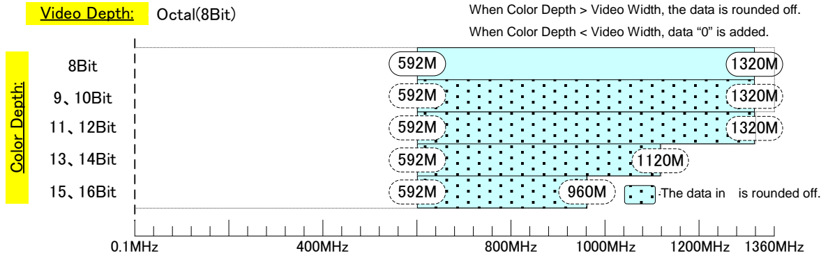
Restrictions on dot clock frequency for4K2K( iTMS)(DVI MODE/Octal Link)
