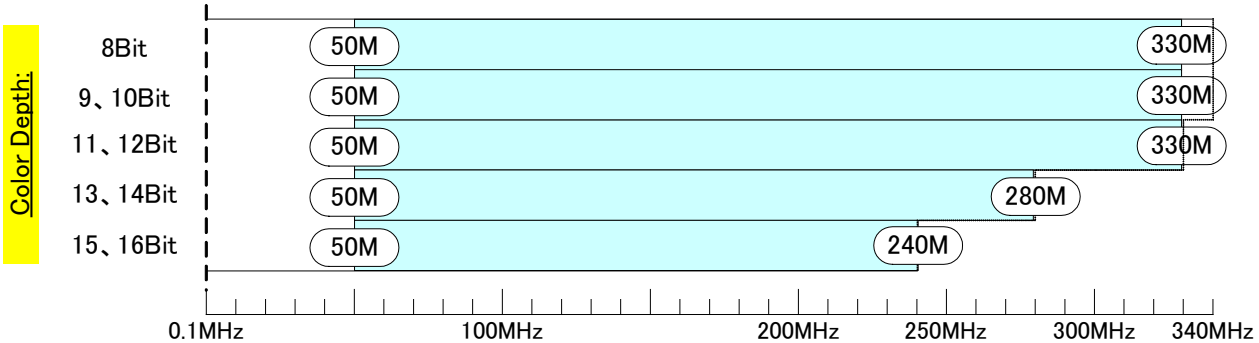
Restrictions on dot clock frequency for 4K2K( iTMDs) (DVI MODE/Dual Link)
