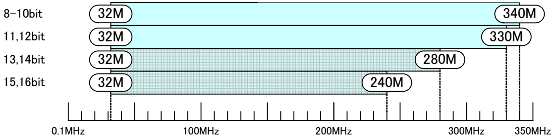
Restrictions on Dot Clock Frequency for DP1, DP2(Dual Mode)
