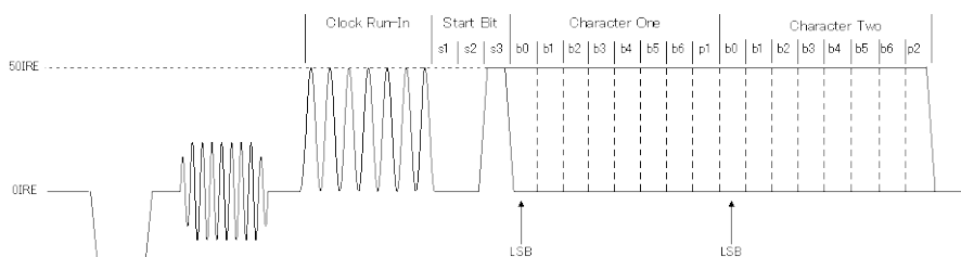
Closed Caption / V-Chip (21Line System)
